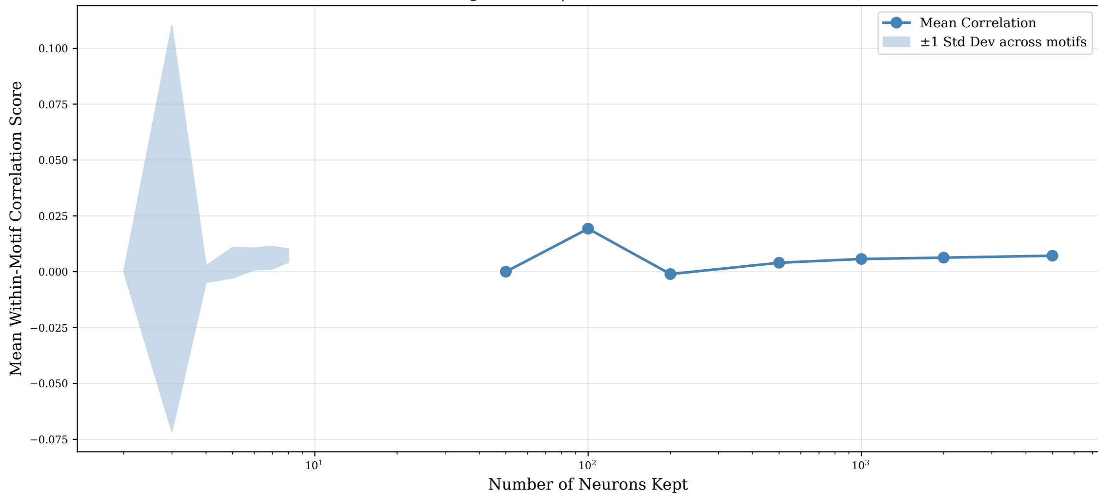
Mean Correlation Score vs Downsampling Level (min_length=5)
